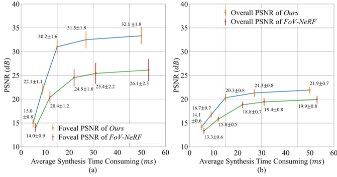
Fig. 9. Ablation experiment results. We visualize PSNR of Ours and FoV-NeRF as a function of the synthesis performance in office in the foveal region (a) and in the overall screen space (b). The average synthesis time consuming of our method is 5.63 ms, 9.23 ms, 15.57 ms, 27.81 ms, 50.31 ms, where \sigma is set to 3.9, 3.3, 2.6, 2.0, 1.4, and N is set to 32, 48, 64, 80, 96. The average synthesis time consuming of FoV-NeRF is 6.31 ms, 12.47 ms, 22.51 ms, 31.73 ms, 53.71 ms, where the number of spheres in the egocentric neural representation is set to 16, 40, 64, 88, 112, and the parameter of each layer in the radiance encoder is set to 64, 128, 256, 512, 1024.
