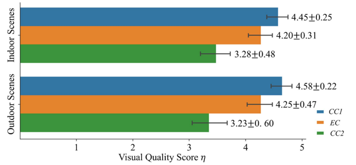
Fig. 10. The visual quality score \eta of the participants in Task 1. X-axis shows the average values and standard deviations of \eta of each pair. Y-axis lists the pair accordingly.
