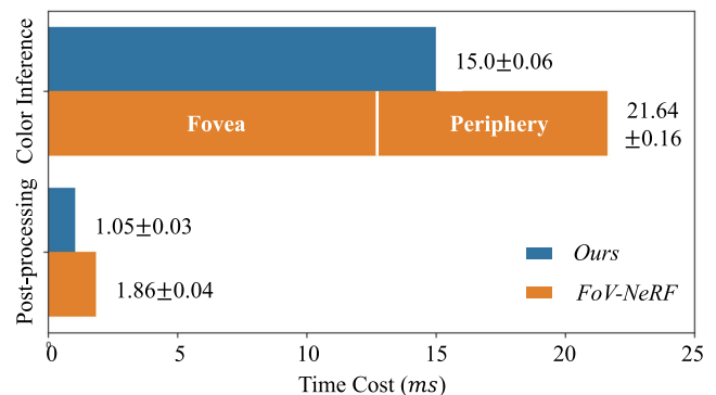
Fig. 8. Performance comparison results. We plot the average time cost of Ours and FoV-NeRF in color inference and post-processing steps in office .
