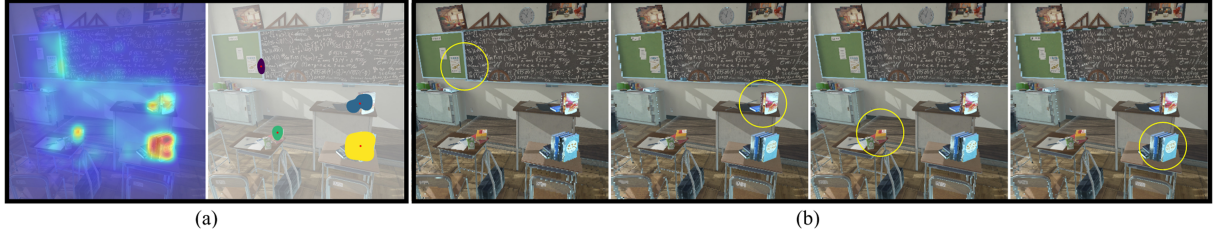
Fig. 3. Gaze position determination in network training. We first estimate the saliency of captured scene images in (a) left, and determine the most likely gaze positions in (a) right based on the saliency estimation. We visualize the synthesized foveated images at the given view with four determined gaze positions in (b).
