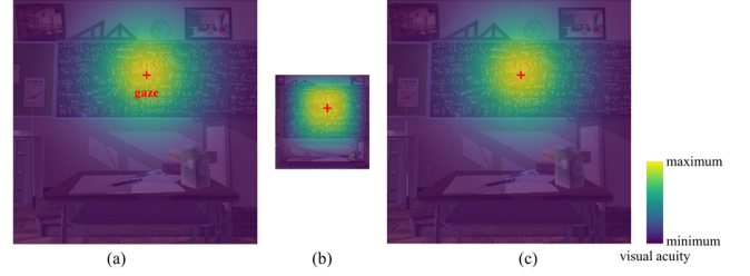
Fig. 4. Stretching and squeezing visualization of synthesis. We visualize the ground truth image in (a) where the gaze is at the center of the image. In (a), the visual acuity decreases from the maximum at the center of fovea to the minimum at the edge of periphery according to the visual acuity fall-off model. (b) is the output result of the uniform-space foveated pixel sampler module in the US-FNRF, and (c) is the final synthesized result of the US-FNRF.
