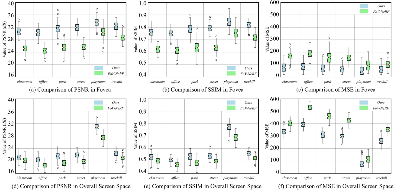
Fig. 5. Synthesis quality quantitative comparison results. We compare the synthesis quality between Ours and FoV-NeRF in the foveal region and overall screen space in all test scenes by the quantitative metrics: PSNR, SSIM, and MSE.
