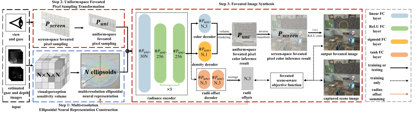
Fig. 2. Overview of our method. The MeNR construction is visualized in the blue dashed box, and the US-FNRF is visualized in the red dashed boxes. In the training process, our method first initializes the MeNR based on the saliency and depth estimation. During the forward propagation process of training, our method performs uniform-space foveated pixel sampling in the MeNR, then feeds the sampling points to the radiance coder and goes through other necessary modules to synthesize the foveated image and outputs the radii offsets of N ellipsoids in x, y, z axes in the MeNR. The radii offsets are then accumulated into the three radii in x, y, z axes of each ellipsoid in the MeNR to complete the forward propagation of this training session. The network is optimized by minimizing the loss calculated by the foveated scene-aware objective function. In the testing process, given the view and gaze position, our method synthesizes the corresponding foveated image in real time.
