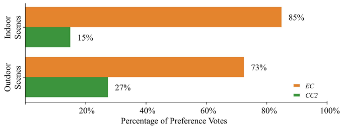
Fig. 11. The participants' preference votes of EC and CC2 in Task 2. X-axis shows the percentage of selecting the condition of each pair. Y-axis lists the pair accordingly.
